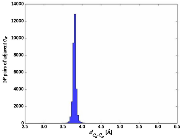
Fig. 3. Histogram for the distance d_{C_{\alpha}-C_{\alpha}} between adjacent alpha-carbon atoms. The distances were calculated from the alpha-carbon atoms coordinates corresponding to a sample of 110 proteins of different length stored at the PDB (31,332 pairs of adjacent alpha-carbon atoms). The mean value and the standard deviation are \langle d_{C_{\alpha}-C_{\alpha}} \rangle = 3.801 \text{ \AA} and \sigma_{C_{\alpha}-C_{\alpha}} = [(d_{C_{\alpha}-C_{\alpha}}^2) - \langle d_{C_{\alpha}-C_{\alpha}} \rangle^2]^{1/2} = 0.061 \text{ \AA} , respectively.
