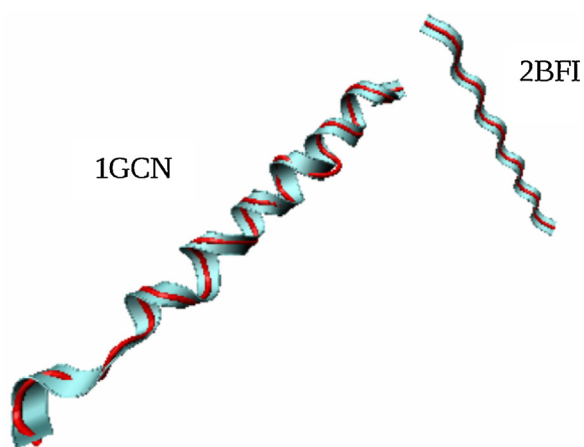
Fig. 5. Trace representation of the alpha-carbon atoms backbone for the small proteins 2BFI and 1GCN. Red (dark grey) tube: from the coordinates obtained using our procedure. Cyan (light grey) ribbon: from the coordinates stored at PDB. (For interpretation of the references to color in this figure legend, the reader is referred to the web version of this article.)
