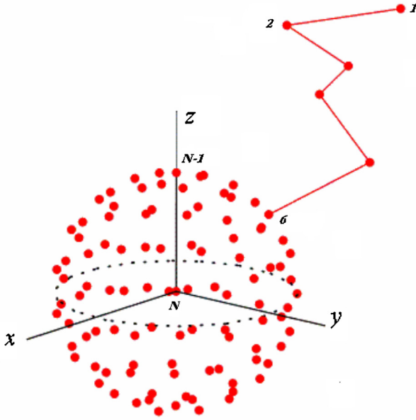
Fig. 4. Development of the alpha-carbon atoms backbone of a hypothetical protein of length N from its position on the sphere surface into its spatial configuration (schematic). The last two alpha-carbon atoms, as well as some of the first ones, are labeled by their order number inside the sequence.
