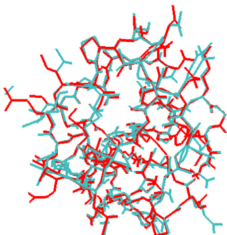
Fig. 11. Full atom line representation of the protein 1HG7. Red (dark grey): reconstruction from the alpha-carbon atoms backbone coordinates (obtained with our procedure) using the method of Rotkiewicz and Skolnick (2008). Cyan (light grey): from the coordinates stored at PDB. In the rebuilt protein the hydrogen atoms do not appear. (For interpretation of the references to color in this figure legend, the reader is referred to the web version of this article.)
