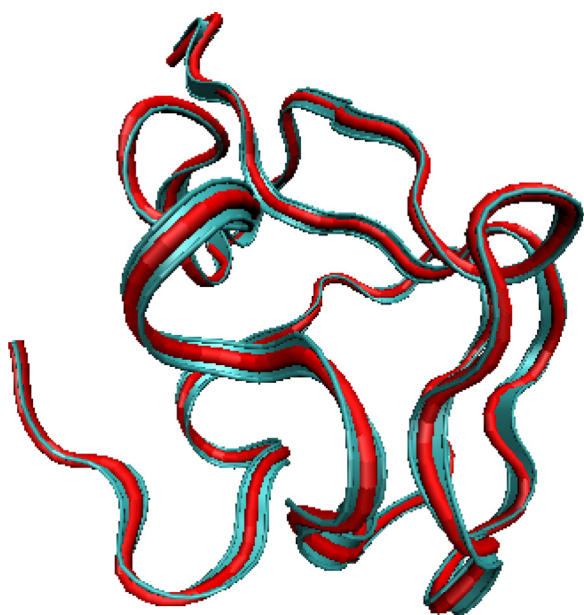
Fig. 7. Trace representation of the alpha-carbon atoms backbone for the protein 1HG7. Red (dark grey) tube: from the coordinates obtained using our procedure. Cyan (light grey) ribbon: from the coordinates stored at PDB. (For interpretation of the references to color in this figure legend, the reader is referred to the web version of this article.)
