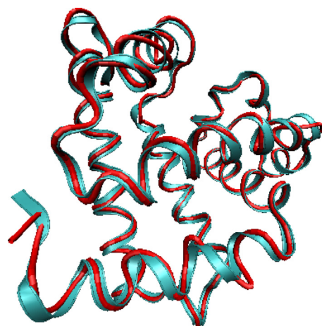
Fig. 8. Trace representation of the alpha-carbon atoms backbone for the protein 1MBN. Red (dark grey) tube: from the coordinates obtained using our procedure. Cyan (light grey) ribbon: from the coordinates stored at PDB. (For interpretation of the references to color in this figure legend, the reader is referred to the web version of this article.)
