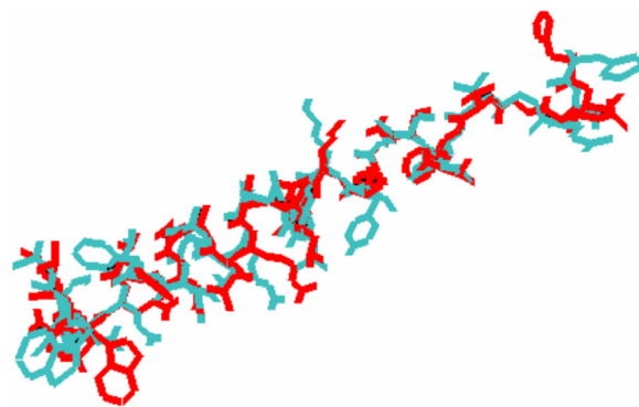
Fig. 10. Full atom line representation of the protein 1GCN. Red (dark grey): reconstruction from the alpha-carbon atoms backbone coordinates (obtained with our procedure) using the method of Rotkiewicz and Skolnick (2008). Cyan (light grey): from the coordinates stored at PDB. In the rebuilt protein the hydrogen atoms do not appear. (For interpretation of the references to color in this figure legend, the reader is referred to the web version of this article.)
