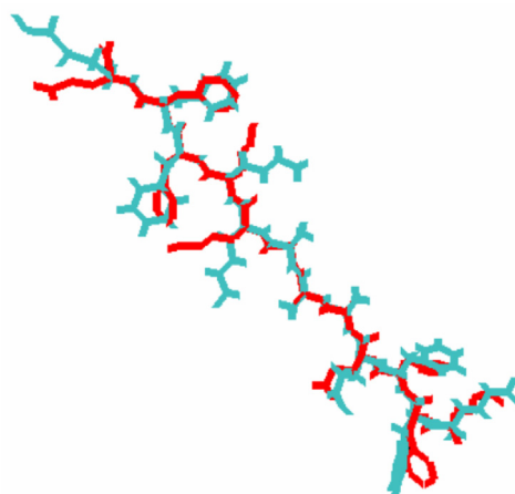
Fig. 9. Full atom line representation of the peptide 2BFI. Red (dark grey): reconstruction from the alpha-carbon atoms backbone coordinates (obtained with our procedure) using the method of Rotkiewicz and Skolnick (2008). Cyan (light grey): from the coordinates stored at PDB. In the rebuilt protein the hydrogen atoms do not appear. (For interpretation of the references to color in this figure legend, the reader is referred to the web version of this article.)
