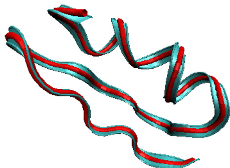
Fig. 6. Trace representation of the alpha-carbon atoms backbone for the protein 2CK5. Red (dark grey) tube: from the coordinates obtained using our procedure. Cyan (light grey) ribbon: from the coordinates stored at PDB. (For interpretation of the references to color in this figure legend, the reader is referred to the web version of this article.)
