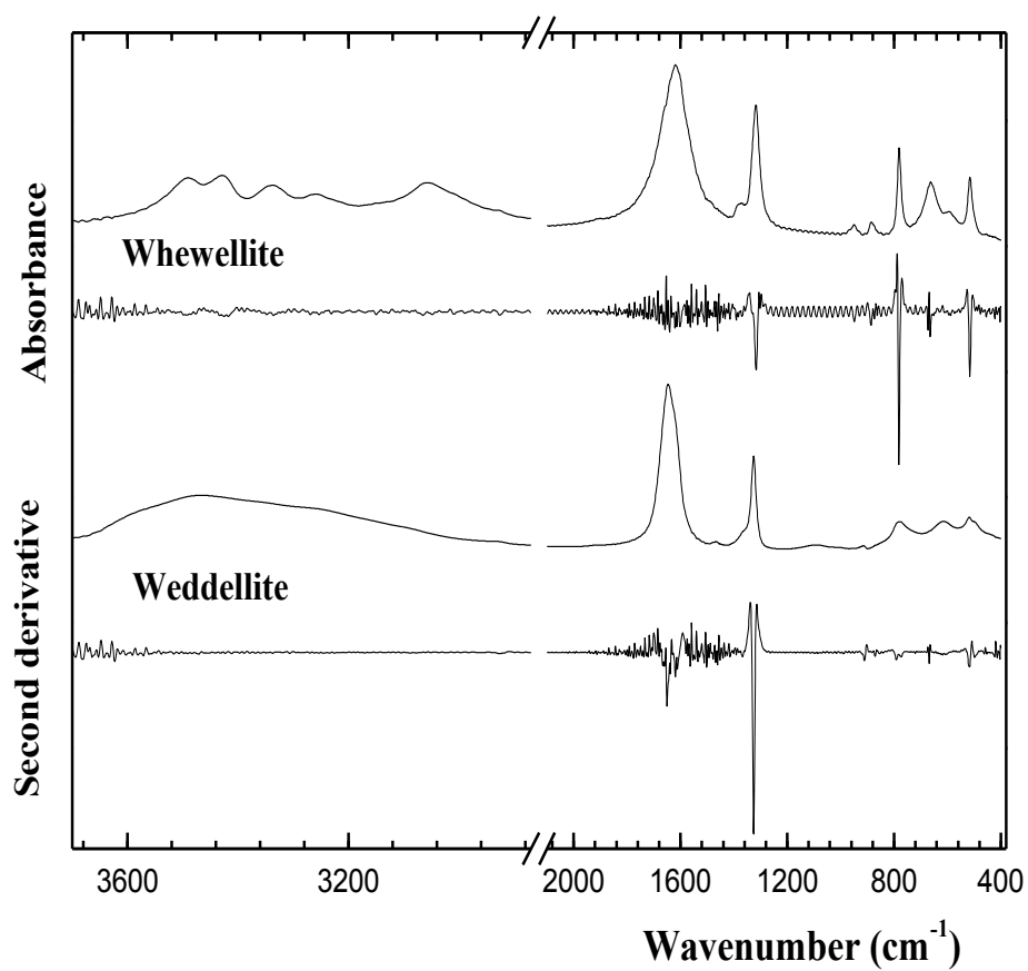
Supplementary Fig. 1 . Infrared spectra in absorbance of whewellite and the weddellite and the corresponding second derivative spectra in wide wavenumber regions
