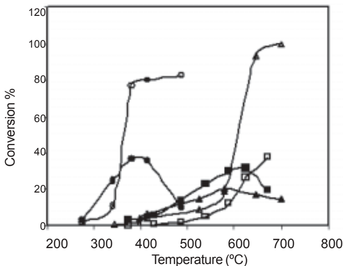
Figure 8: NO-N_2 conversion of CLI ( \blacktriangle ), Co-CLI ( \blacksquare ) and Rh-Co-CLI ( \bullet ). Corresponding data for the C_3H_8-CO_2 conversion are indicated by empty symbols.
