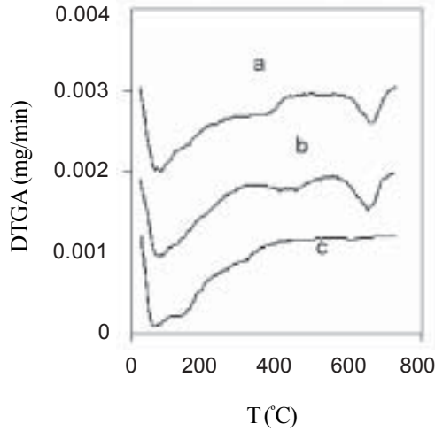
Figure 2: DTGA plots of: a) \text{NH}_4\text{-CLI} , b) \text{Co-CLI} , c) \text{CLI}
