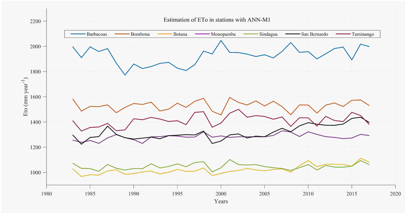
Figure 5: Estimation of ETo by ANN-M1 at stations with scarce information
