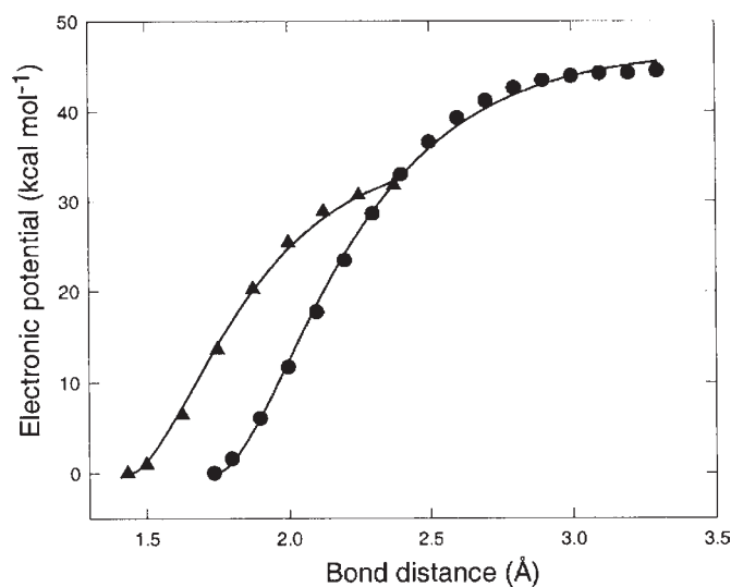
Figure 4. Potential energy curves for FS(O_2)OCl \rightarrow FS(O_2)O + Cl (●) and FS(O_2)OF \rightarrow FS(O_2)O + F (▲) calculated at the BAC-G3MP2B3 level. The solid lines are the fits with Morse functions (see text).
