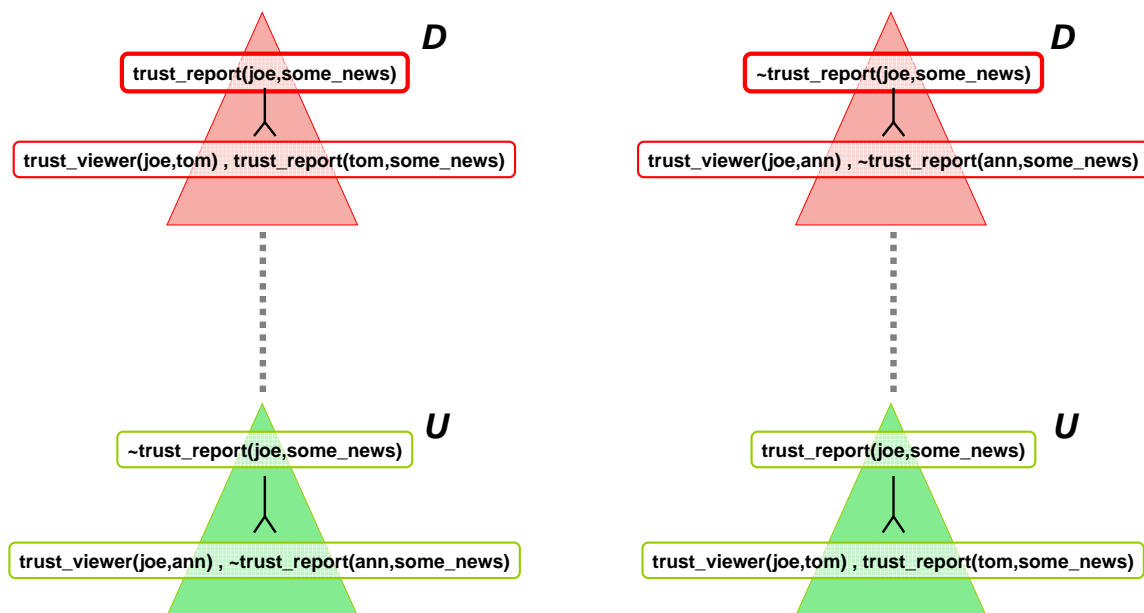
Figure 4: DeLP dialectical trees showing that it is not possible to conclude that the “Some News” report should be trusted or distrusted by Joe and therefore it will be classified as undecided.
