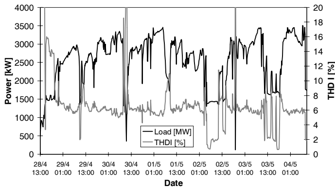
Fig. 16: Profile of THD I [%] and power.
