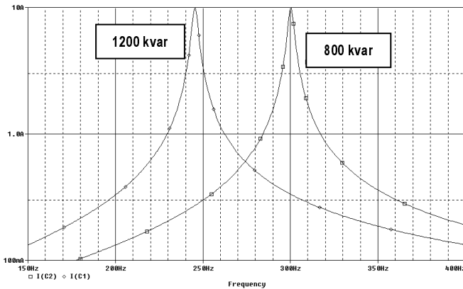
Fig. 13: System frequency responses for the two values of capacitance: 1200 and 800 kvar capacitors.
