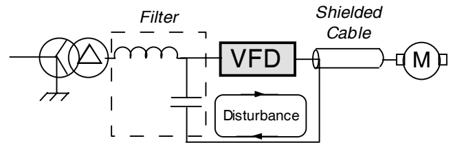
Fig. 9: Solution to mitigate the common-mode voltage.
