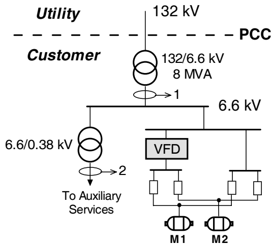
Fig. 3: Simplified one-wire diagram of the plants.
