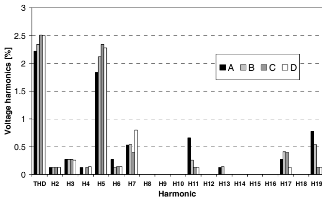
Fig. 20: Harmonics recorded in the four plants.
