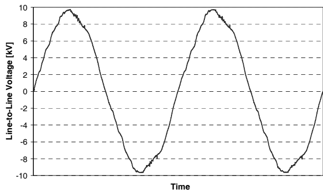
Fig. 6: Waveform of line-to-line voltage at 6.6 kV.
