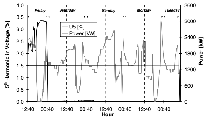
Fig. 15: 5 th harmonic voltage and power taken by the plant.
