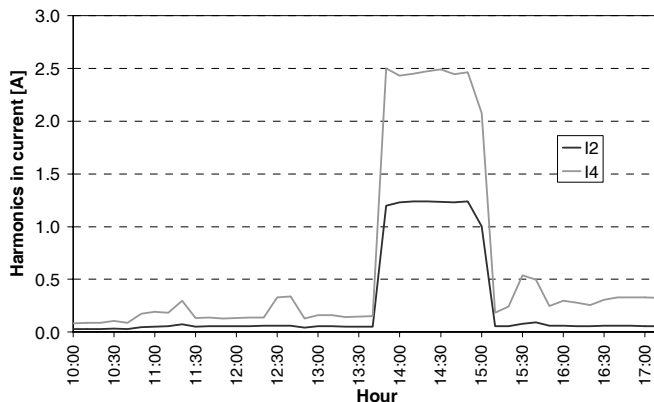
Fig. 11: Trend of 2 nd and 4 th harmonic current.
