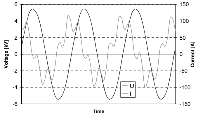
Fig. 12: Waveform of voltage and current with the VFD connected but not operating.
