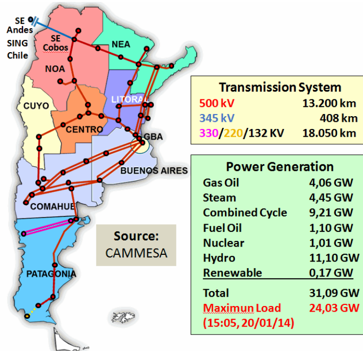
Figure 1. Argentinean Interconnected System (SADI). 345 kV line (blue) between Cobos (SADI-Argentina) and Andes (SING-Chile).
