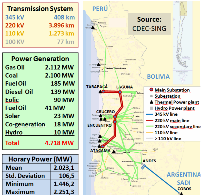
Figure 2. Chile North Power System (SING). 345 kV line (blue) between Cobos (SADI-Argentina) and Andes (SING-Chile).
