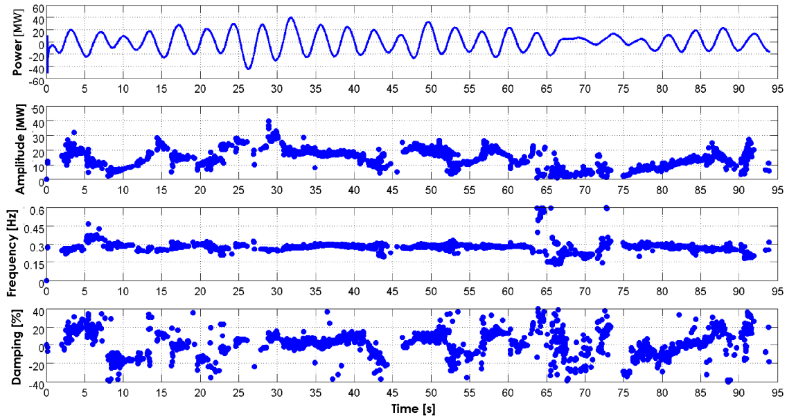
Figure 10: Prony Analysis. Power SING \rightarrow SADI \cong 50 MW.
