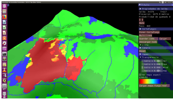
Figure 6: Same simulation step than the previous figure but with a firebreak (white line) at the top left corner. The fire does not spread to the north of the terrain. Cellular Automaton was executed 460 times.
