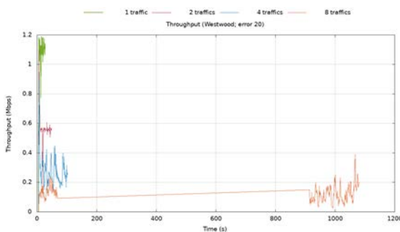
Fig. 30 Throughput vs. Time – 20 errors
